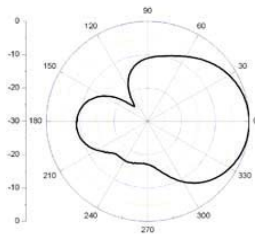
H Plane(72° )
